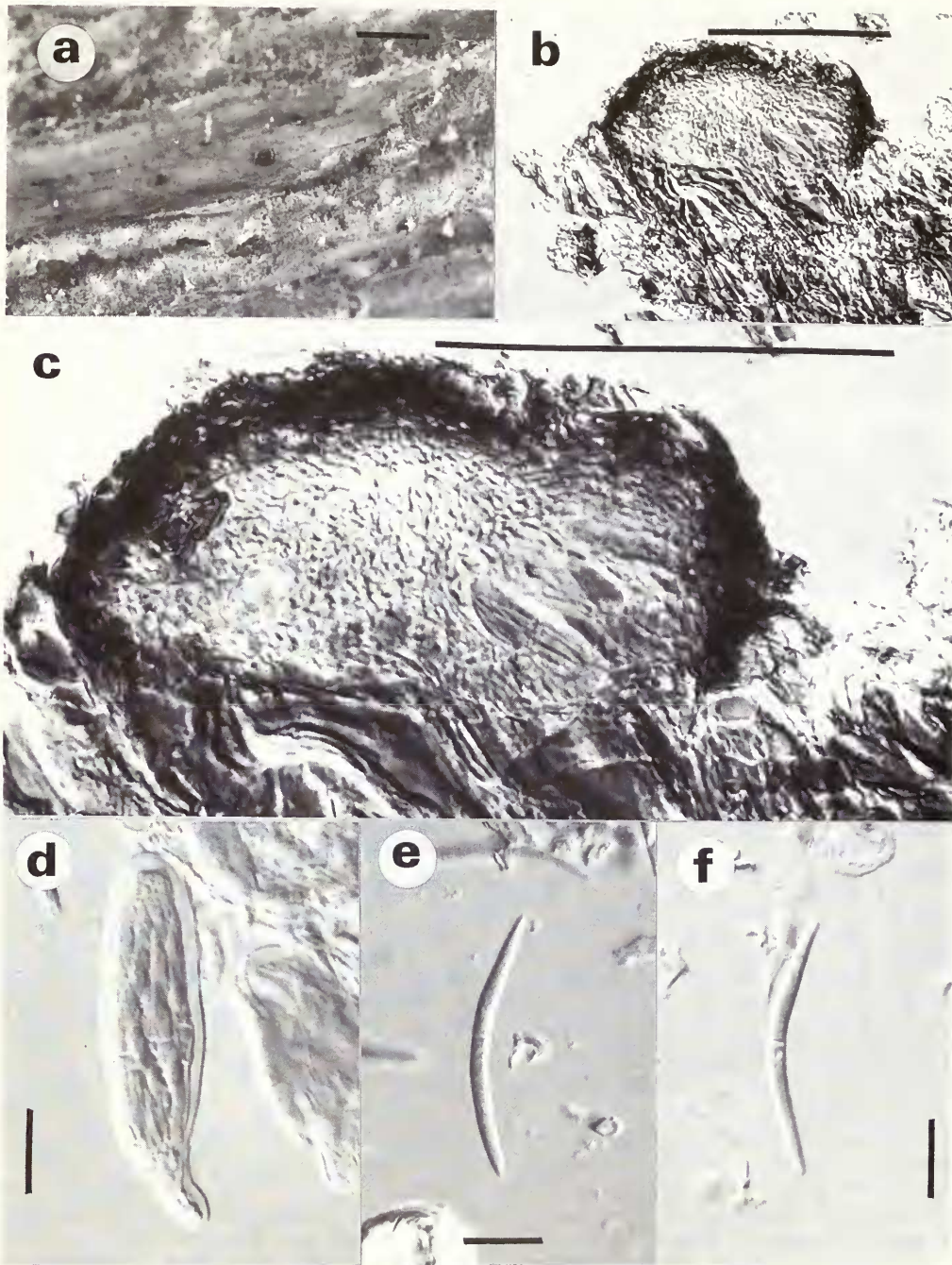
Fig. 10 Leptorhaphis laricis (Lahm) Aguirre (B 37536–holotype) (a) Surface view; scale = 500 µm; (b), (c) Vertical sections of ascomata; scale = 100 µm; (d) Ascus and ascospores; (e), (f) Ascospores; scale = 10 µm.
